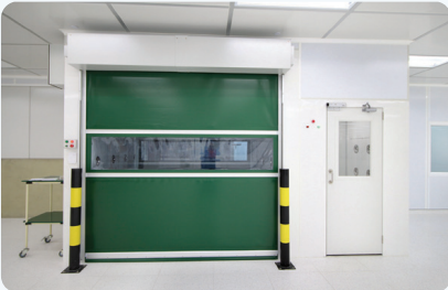
Air Showers
